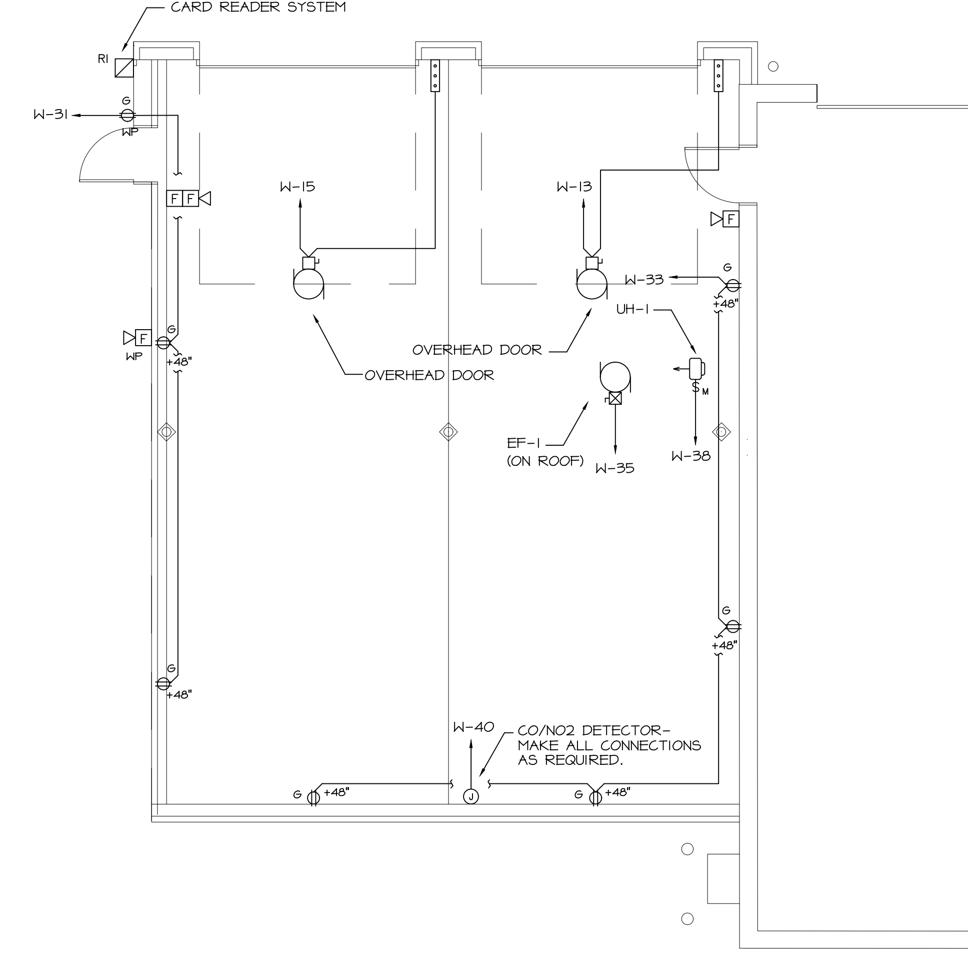
FLOOR PLAN - POWER AND SYSTEMS ALT #1 ADDITION SCALE: 3/16"=1'-0"
